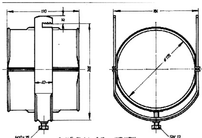
Type C For anchor bar (18-22mm slot)
