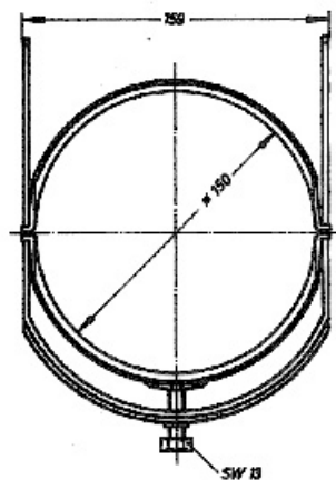
Type C For anchor bar (18-22mm slot)
