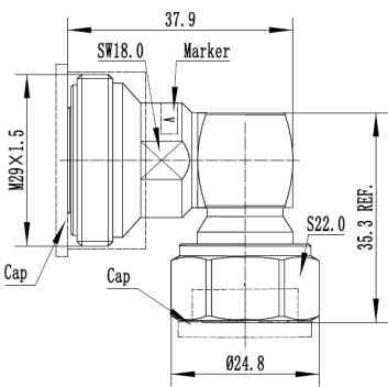
Coaxial Adapter 7-16 Female - 4.3-10 Male with right angle
