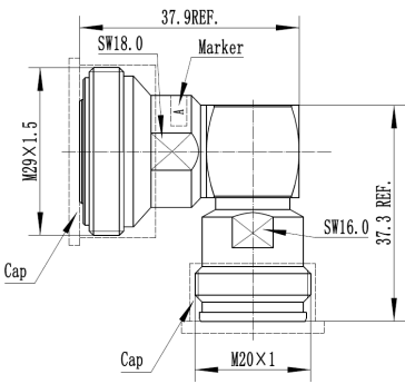
Coaxial Adapter 7-16 Female - 4.3-10 Female with right angle
