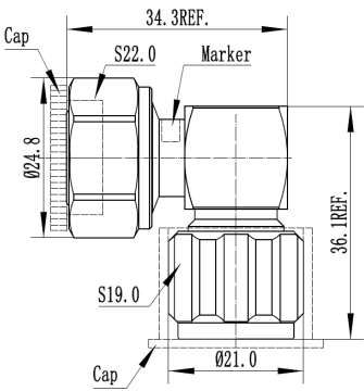
Coaxial Adapter 4.3-10 male, right angle - N Male
