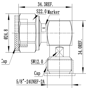
Coaxial Adapter 4.3-10 male, right angle - N female
