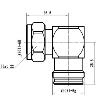
Coaxial Adapter, 4.3-10 Male/Female Right Angle
