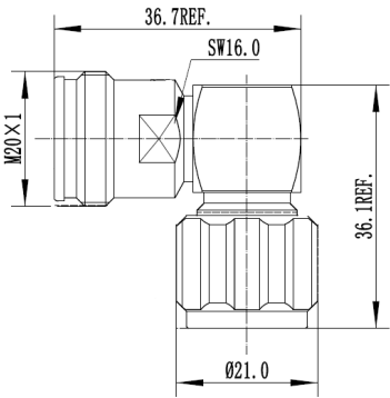
Coaxial Adapter 4.3-10 Female - N Male with right angle
