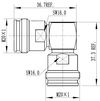
Coaxial Adapter 4.3-10 Female - 4.3-10 Female with right angle
